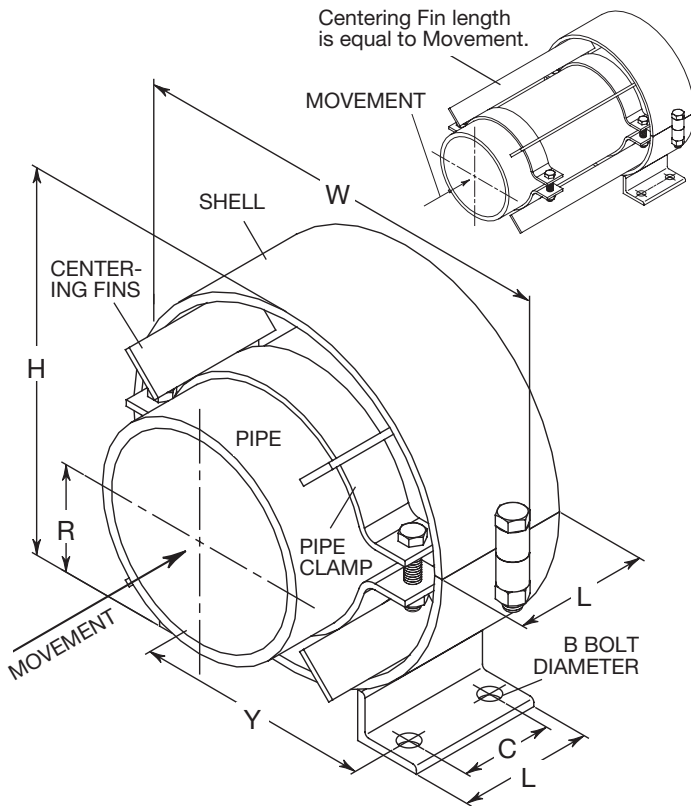
SPG DIMENSIONS (inches)
